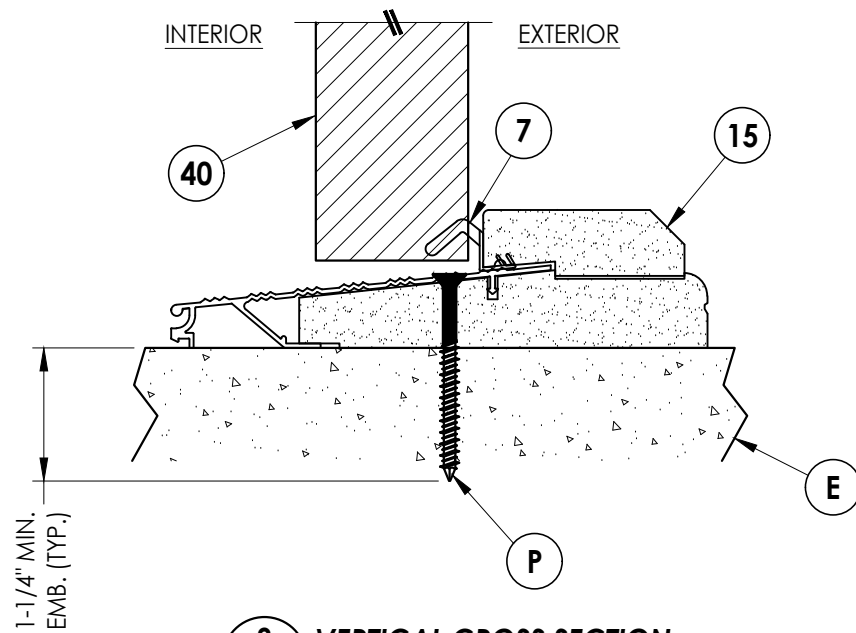
3 VERTICAL CROSS SECTION 10 Outswing Sill
