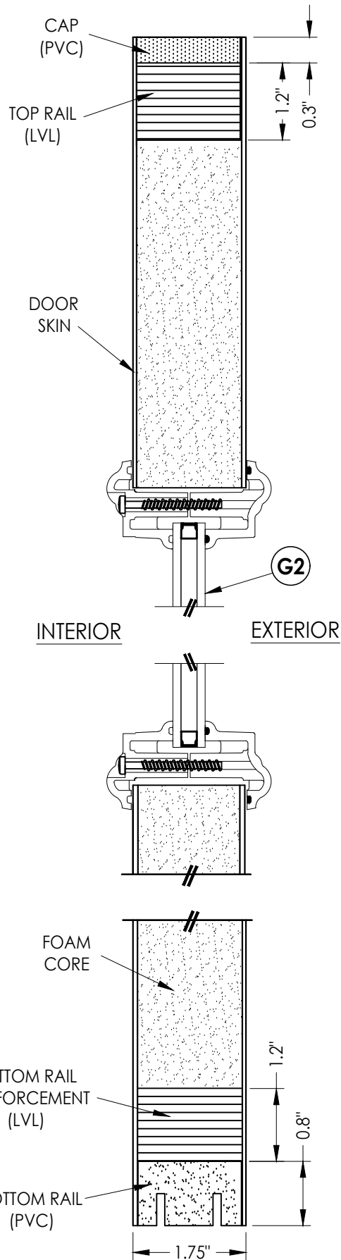
2 4 VERTICAL CROSS SECTION
