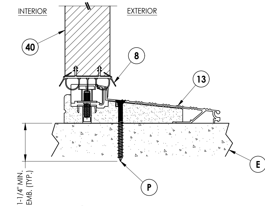
1 VERTICAL CROSS SECTION 10 Inswing Sill
