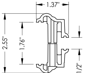
4A RSL LITE FRAME INJECTION MOLDED
