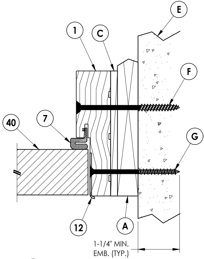
2 8 HORIZONTAL CROSS SECTION Outswing Shown (Inswing Similar) Shown w/ 1X Buck
