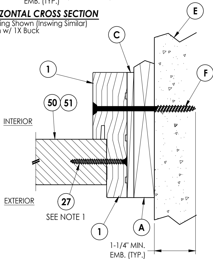
3 8 HORIZONTAL CROSS SECTION Outswing Shown (Inswing Similar) Shown w/ 1X Buck
