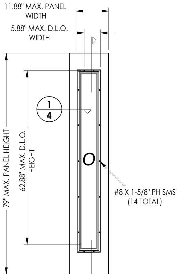
51 FIBERGLASS SIDELITE PANEL Masonite
