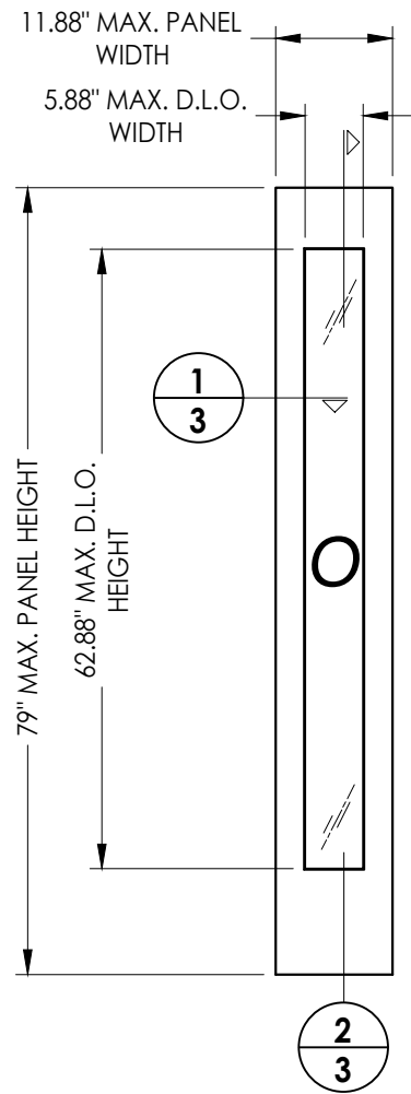
50 FIBERGLASS SIDELITE PANEL Masonite
